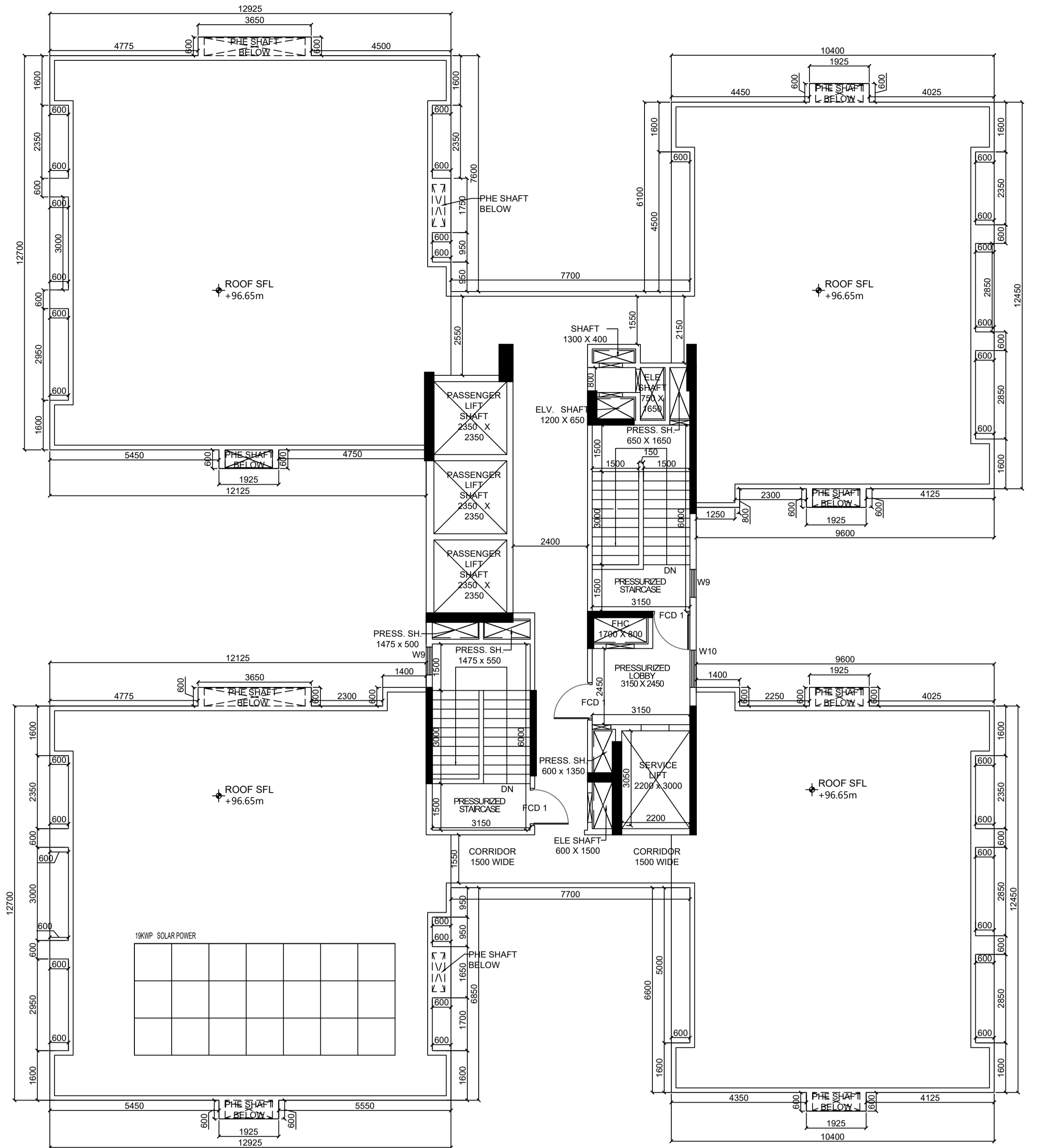
ROOF PLAN
